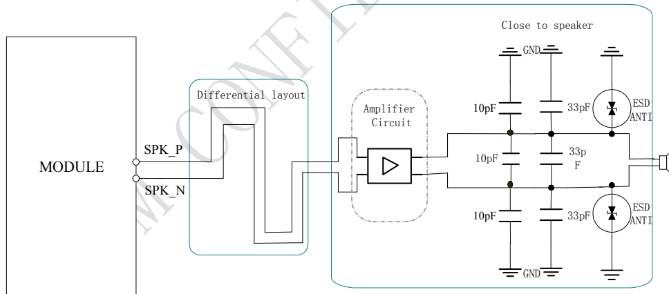
Figure 24: Speaker interface with amplifier configuration
